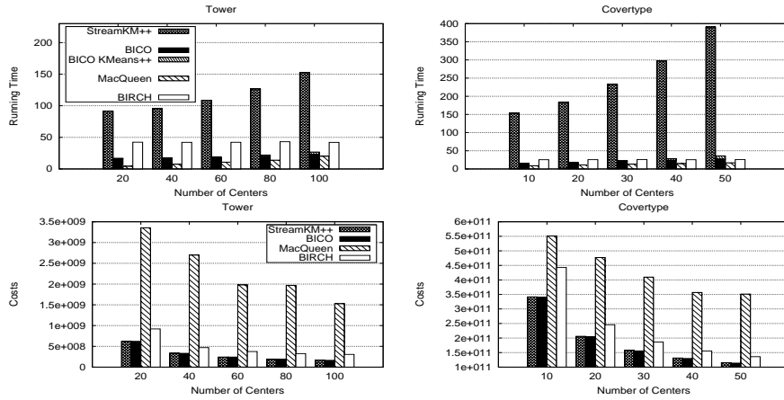
Fig. 4: Running times and costs for datasets Tower and Coverttype
